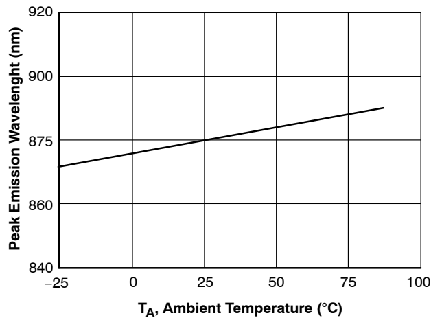
Figure 3. Peak Emission Wavelength vs. Ambient Temperature
