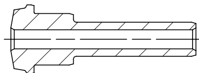
121666-2 FOLLOWER (FOR -05 & -06)
