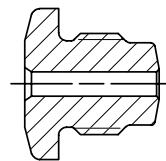
124451 DRIVING ANVIL -04
