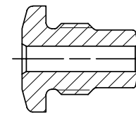
124449 DRIVING ANVIL -06
