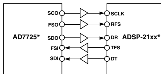
Figure 35. AD7725 to ADSP-21xx Interface
