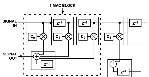
b) FIR Postprocessor Implementation
