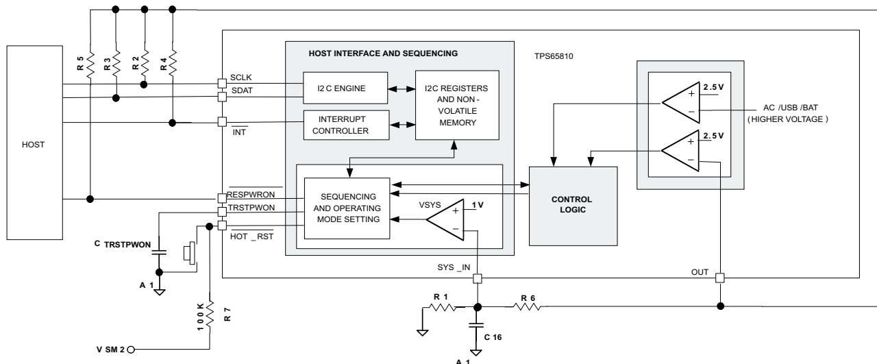
Figure 27. Simplified Block Diagram
