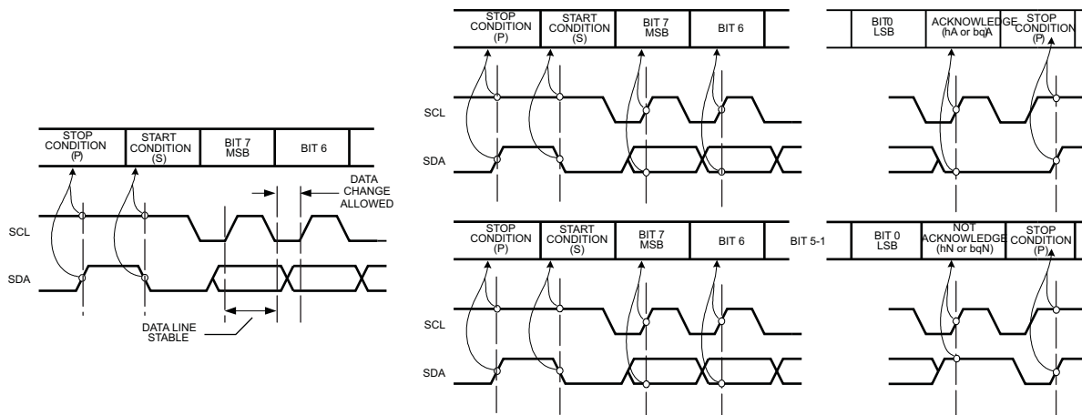
Figure 24. I 2 C operation waveforms
