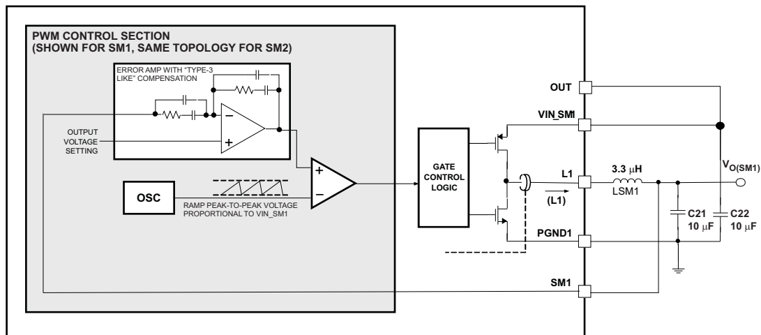
Figure 42. PWM Operation
