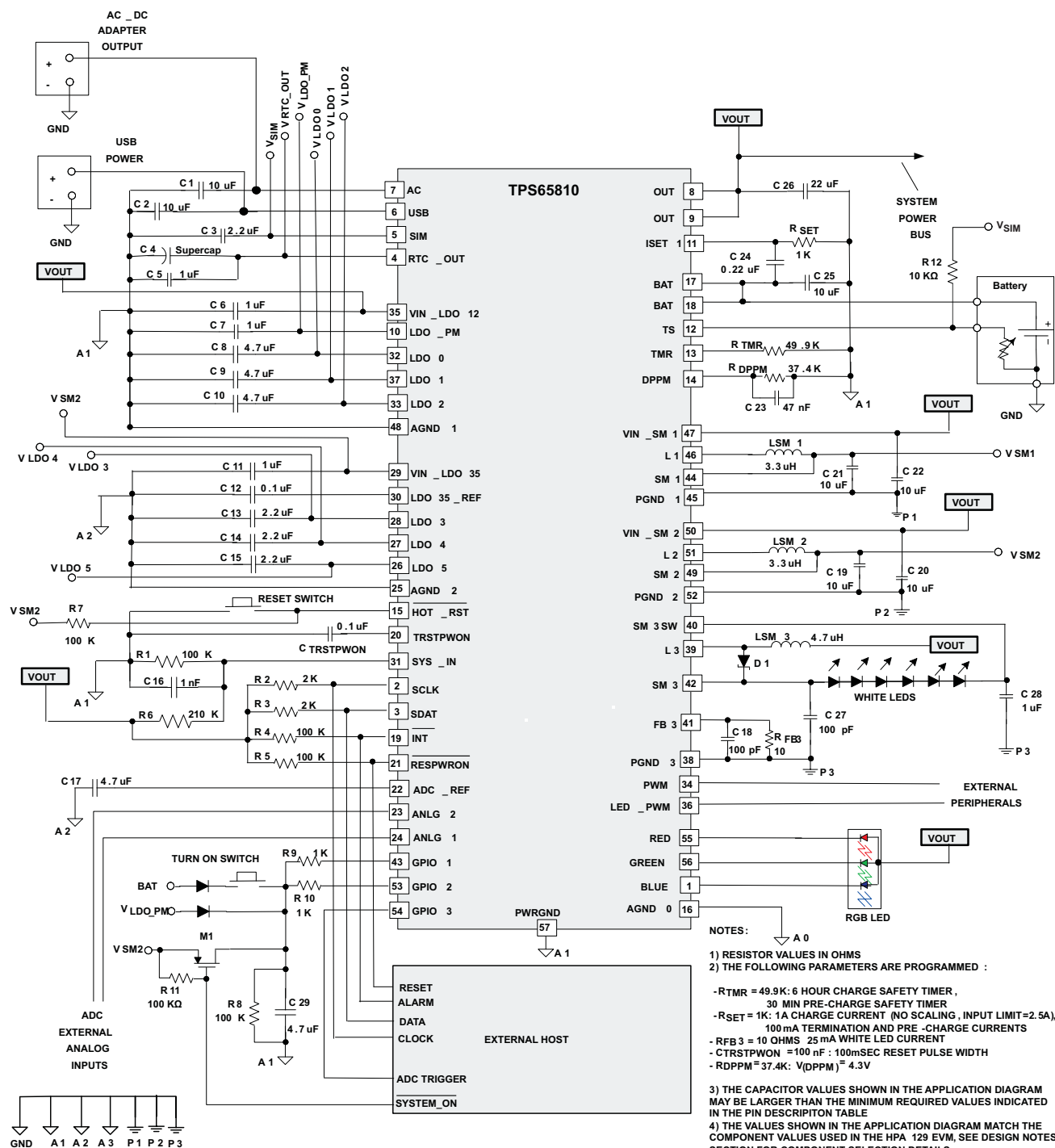
Figure 3. TPS65810 Application Diagram, Recommended External Components
