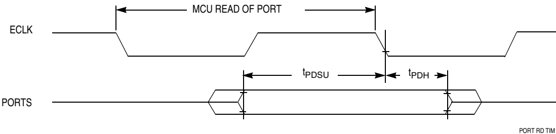
Figure 21-6. Port Read Timing Diagram
