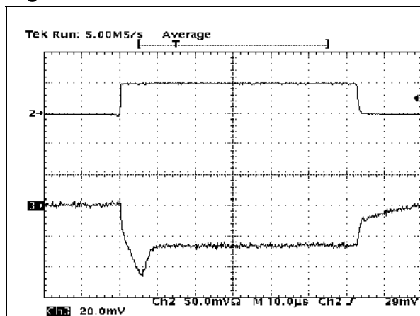
Figure 15. Load transient
