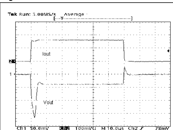
Figure 16. Load transient
