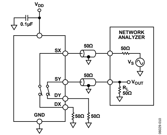
Figure 27. Channel-to-Channel Crosstalk
