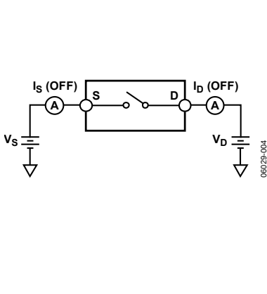
Figure 23. Off Leakage
