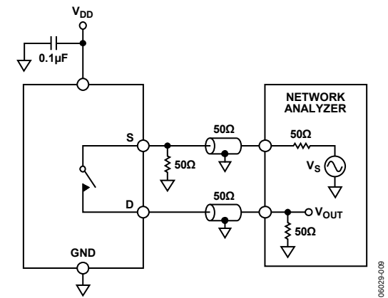
Figure 26. Off Isolation
