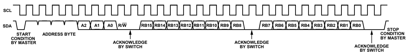
Figure 32. Read Operation
