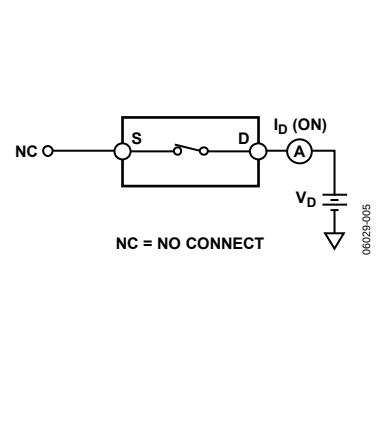
Figure 24. On Leakage
