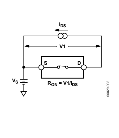
Figure 22. On Resistance
