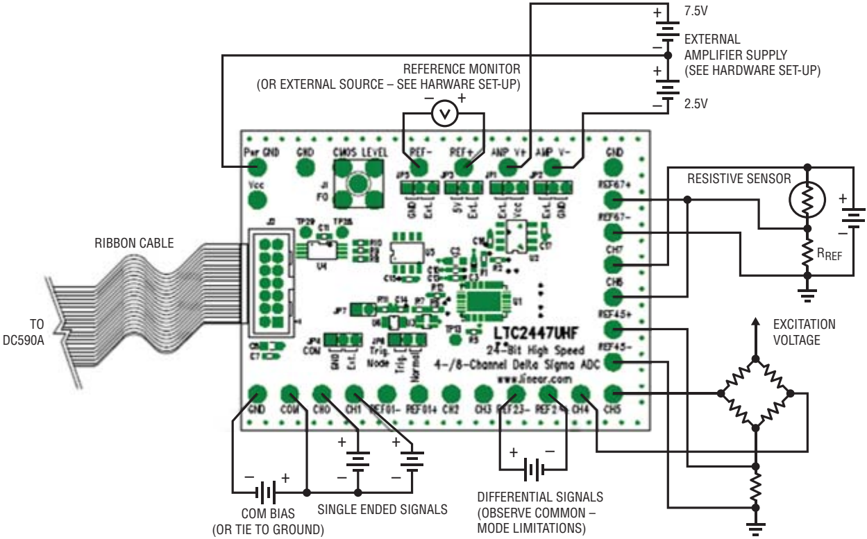
Figure 1. Connection Diagram
