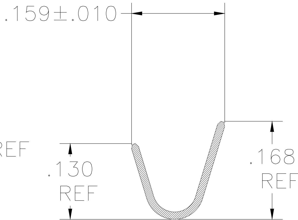
SECTION C-C
