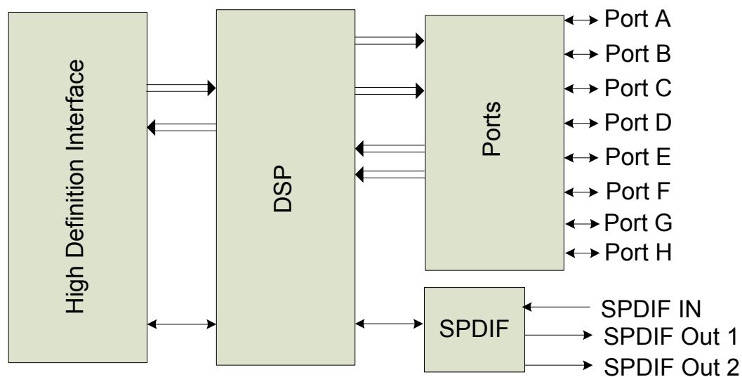
Figure 1. 92HD89D Block Diagram
