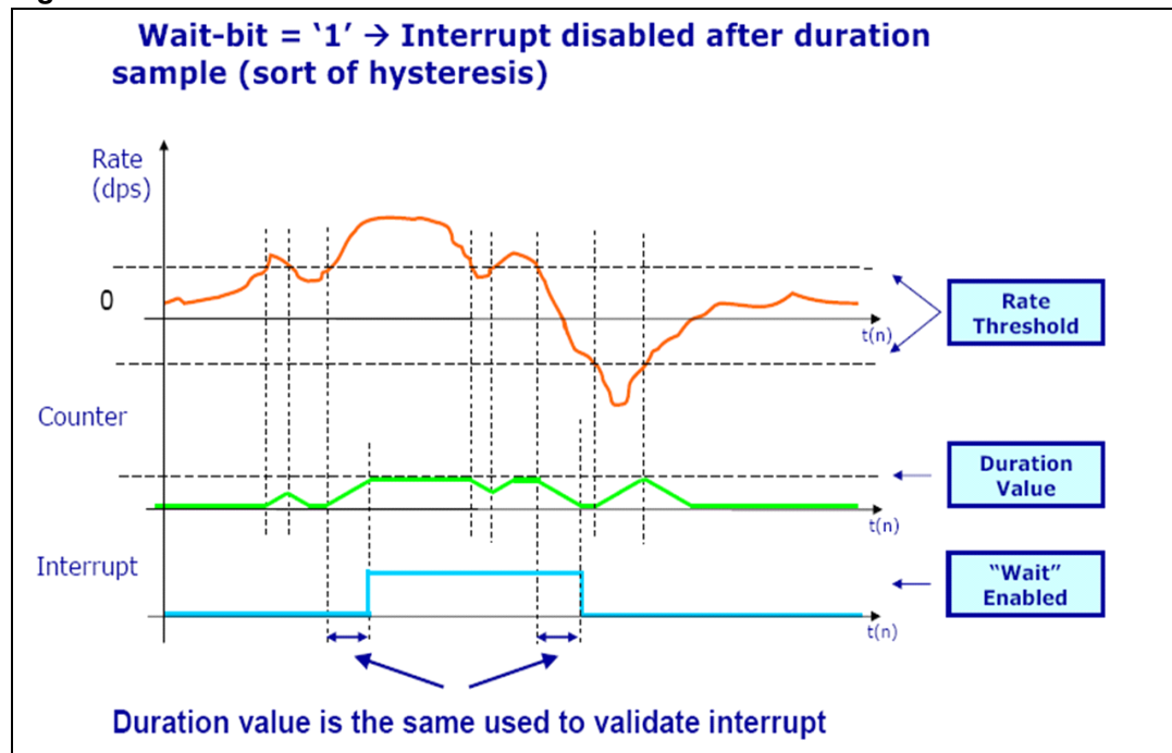
Figure 20. Wait enabled
