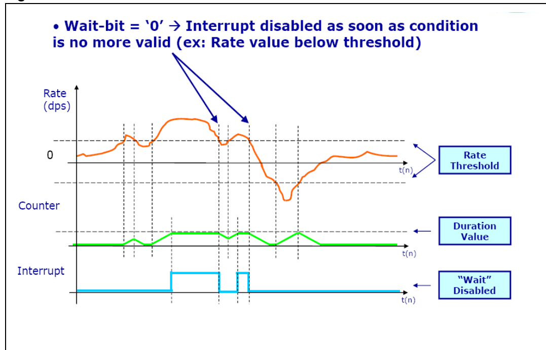
Figure 19. Wait disabled
