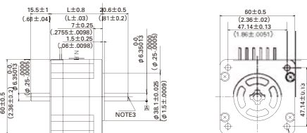
Lead wire type
