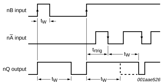
Fig 12. Output pulse control using retrigger pulse n\overline{A}
