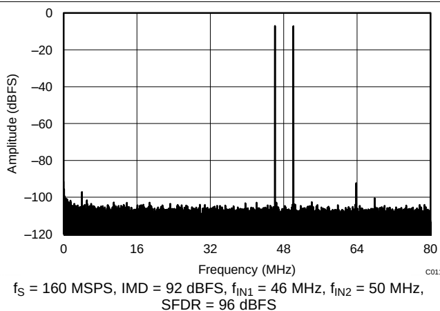
Figure 11. FFT for Two-Tone Input Signal ( -7\text{ dBFS} at 46\text{ MHz} and 50\text{ MHz} )
