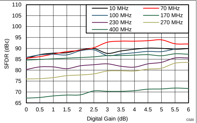
Figure 20. Spurious-Free Dynamic Range vs Digital Gain and Input Frequency
