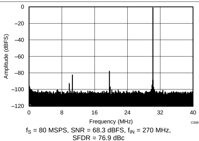
Figure 74. FFT for 270-MHz Input Signal (Dither Off)
