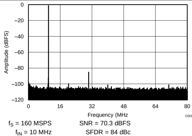
Figure 203. Performance FFT at 10 MHz (Low Input Frequency)
