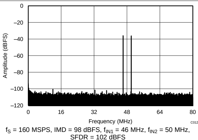
Figure 12. FFT for Two-Tone Input Signal ( -36\text{ dBFS} at 46\text{ MHz} and 50\text{ MHz} )
