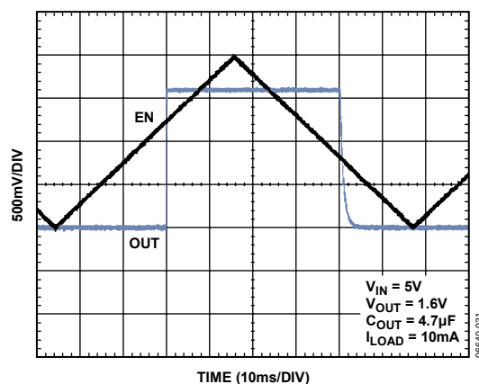
Figure 31. ADP1706 Typical EN Pin Operation
