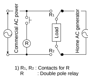
Fig. 4 Bad example of Form A and B use
