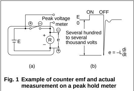
In Fig. 1 (a), an emf ( e = -L \frac{di}{dt} ) with a steep waveform is generated across the coil
