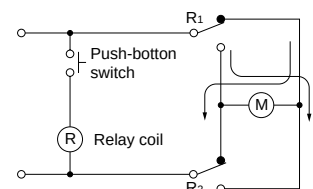
3) R 1 , R 2 : Contacts for R R : Double pole relay
