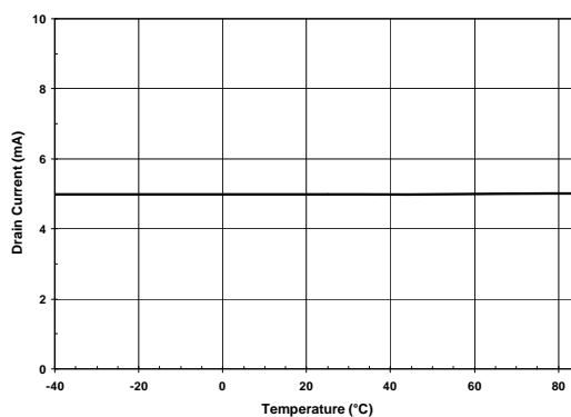
ZABG6002 Drain Current (D3 & D6 only) vs Temperature
