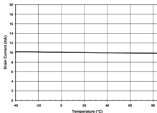
ZABG6002 Drain Current (D1 - D6) vs Temperature
