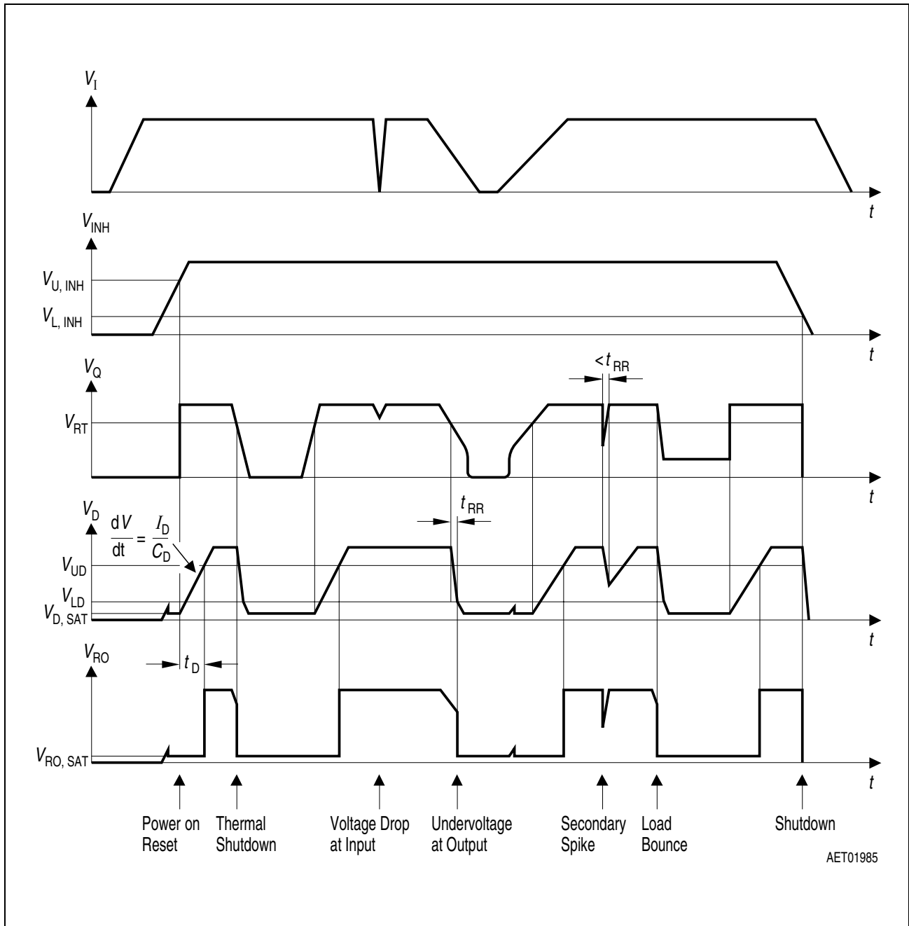
Figure 5 Time Response
