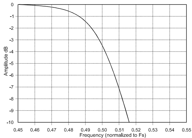
Figure 24. Double-Speed Stopband Rejection
