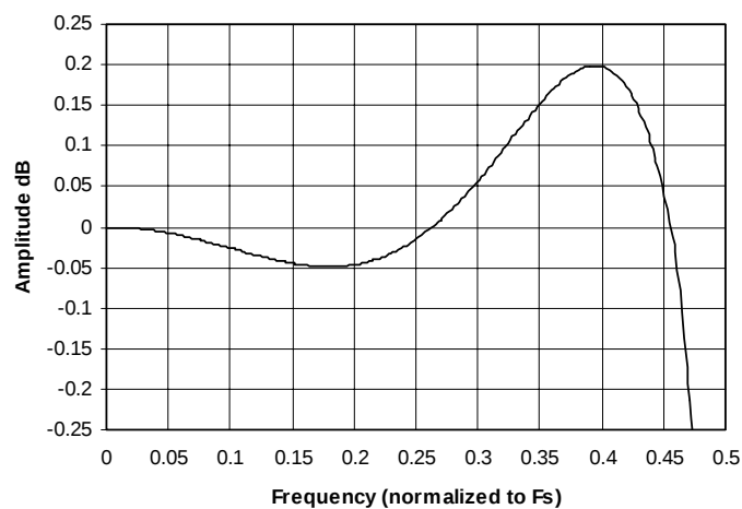
Figure 21. Double-Speed Frequency Response
