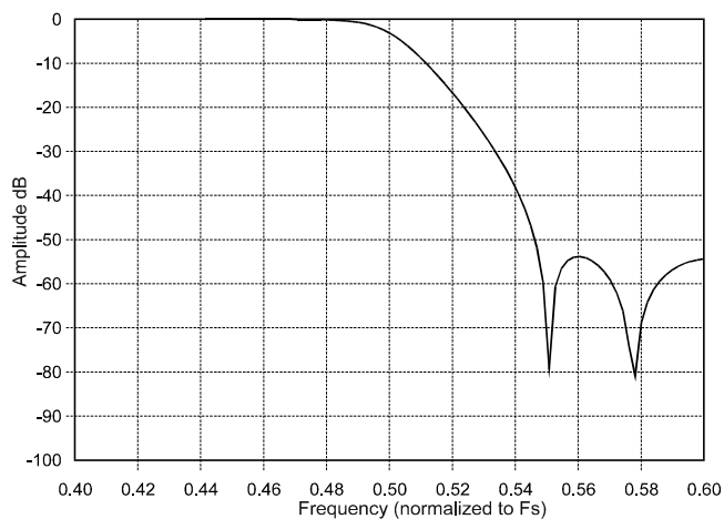
Figure 18. Single-Speed Transition Band
