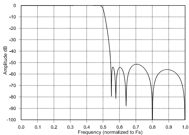
Figure 20. Single-Speed Stopband Rejection
