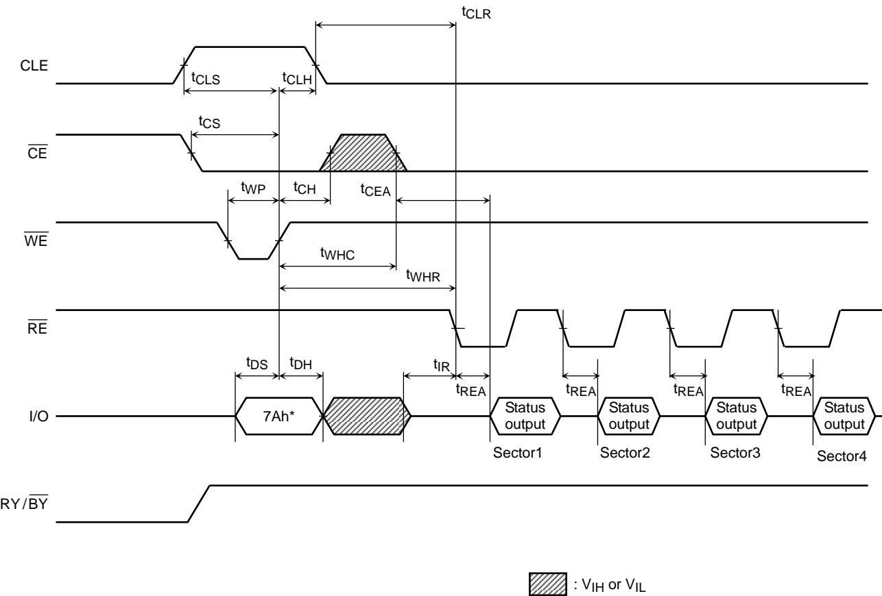
ECC Status Read Cycle Timing Diagram
