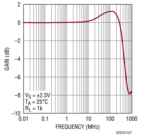
Gain vs Frequency (AV = 1)
