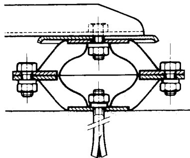
BECA mountings in series (to double the deflection)
