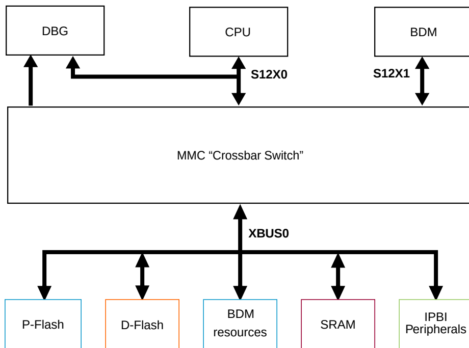
Figure 3-12. S12P platform
