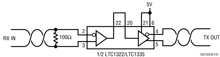
Figure 21. Typical Cable Repeater for RS422 Interface
