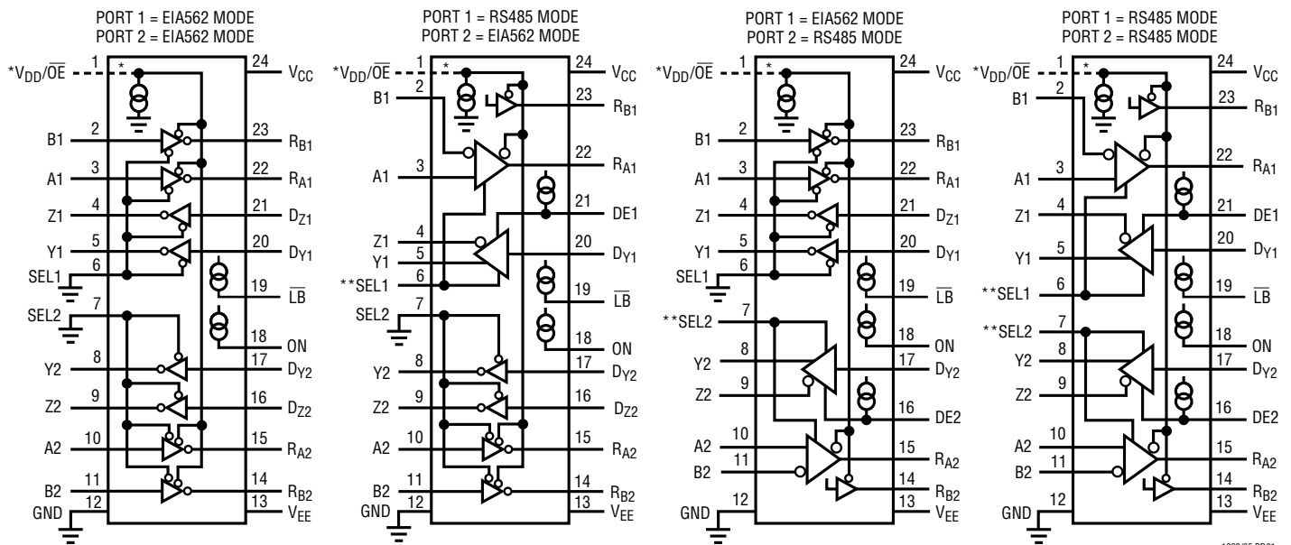
LTC1322/LTC1335 Interface Configuration Without Loopback
