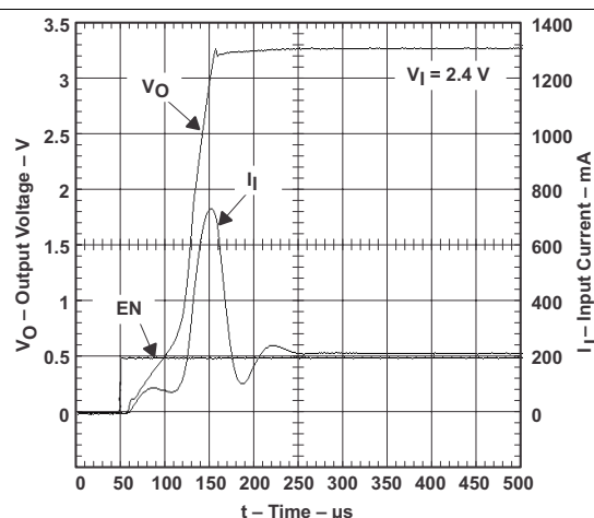
Figure 18. Start-Up Timing
