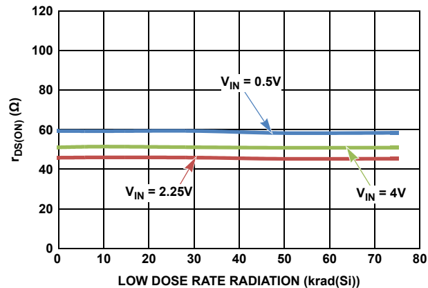
FIGURE 30. r_{DS(ON)} ( V^+ = 4.5V ), GROUNDED
