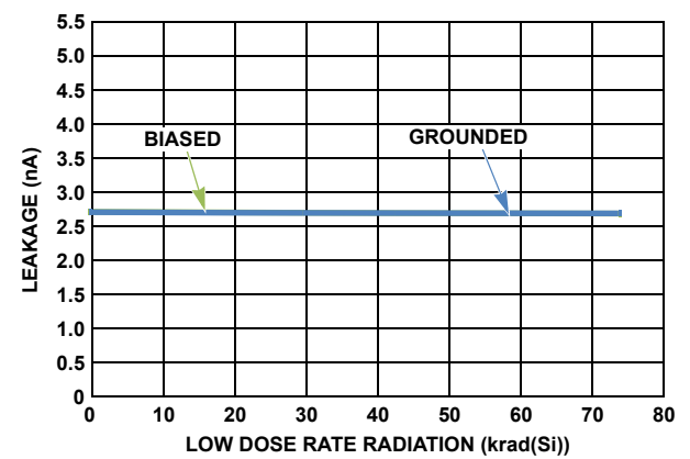
FIGURE 50. I_{S(ON)} ( V^+ = 3.6V , V_{IN} = 7V )
