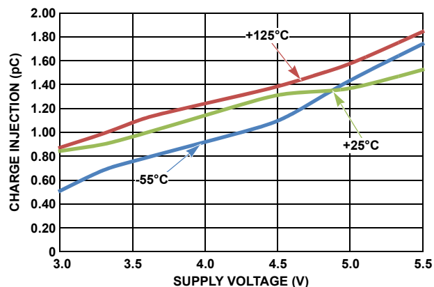
FIGURE 28. CHARGE INJECTION
