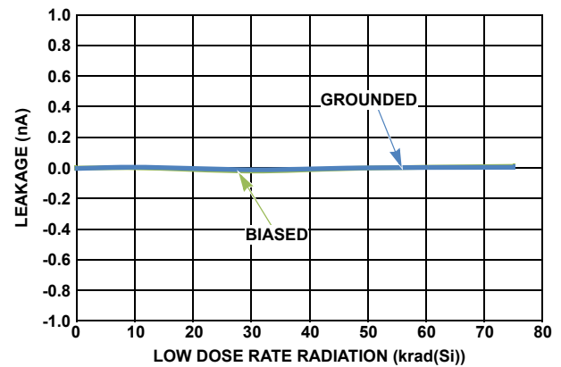
FIGURE 48. I_{S(OFF)} ( V^+ = 3.6V , V_{IN} = 3.1V )
