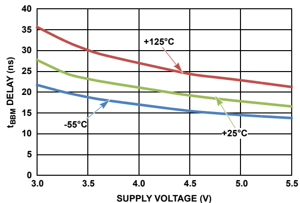
FIGURE 20. BREAK-BEFORE-MAKE DELAY
