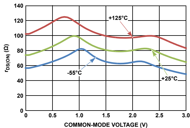
FIGURE 14. r_{DS(ON)} vs COMMON-MODE VOLTAGE ( V^+ = 3V )
