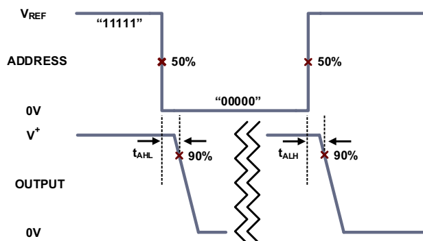
FIGURE 4. ADDRESS TIME TO OUTPUT DIAGRAM
