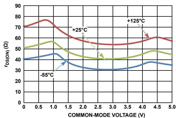
FIGURE 12. r_{DS(ON)} vs COMMON-MODE VOLTAGE ( V^+ = 5V )
