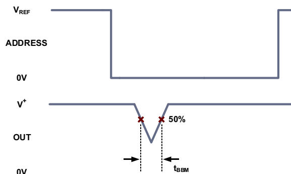
FIGURE 8. BREAK-BEFORE-MAKE DIAGRAM
