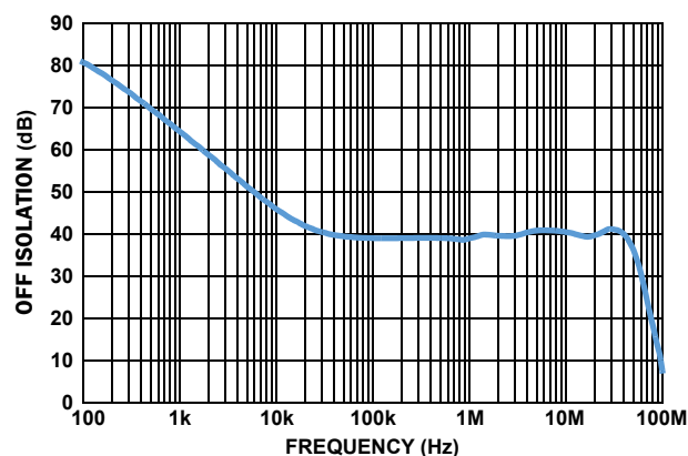
FIGURE 26. OFF ISOLATION ( V^+ = 5V , +25^\circ\text{C} , R_L = \text{OPEN} )
