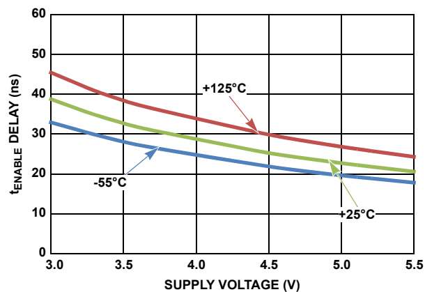
FIGURE 22. ENABLE TO OUTPUT PROPAGATION DELAY
