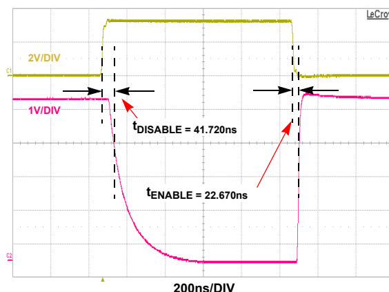
FIGURE 24. ENABLE/DISABLE PROPAGATION DELAY
