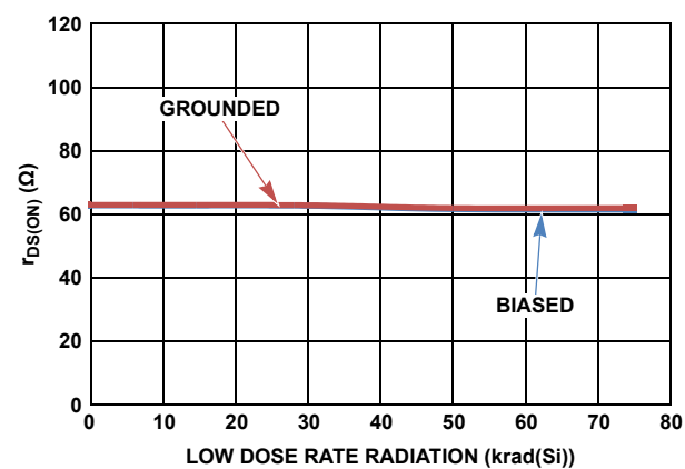
FIGURE 32. r_{DS(ON)} MAXIMUM ( V^+ = 4.5V )
