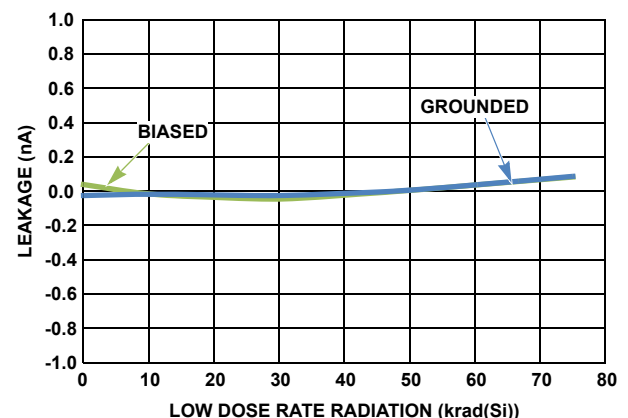
FIGURE 52. I_{D(OFF)} ( V^+ = 3.6V , V_{IN} = 3.1V )
