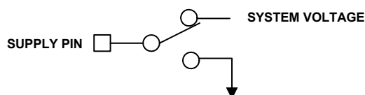
FIGURE 53. COLD SPARING SETUP WITH SUPPLIES SHORTED
