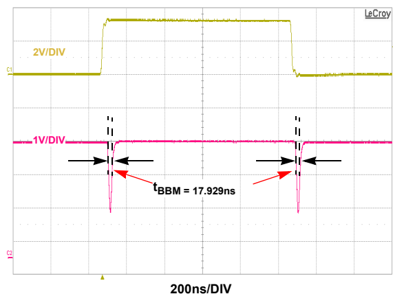
FIGURE 21. BREAK-BEFORE-MAKE DELAY
