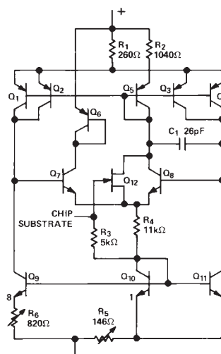
Figure 1. Schematic Diagram
