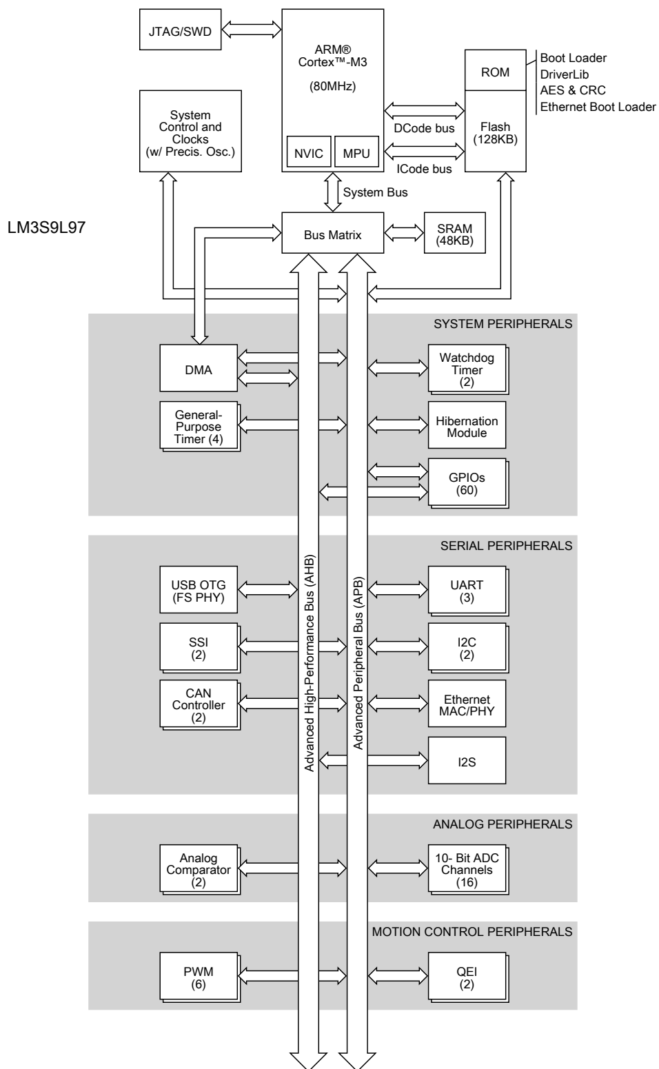
Figure 1-1. Stellaris LM3S9L97 Microcontroller High-Level Block Diagram
