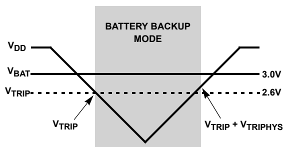
FIGURE 8. BATTERY SWITCHOVER WHEN V_{BAT} > V_{TRIP}
