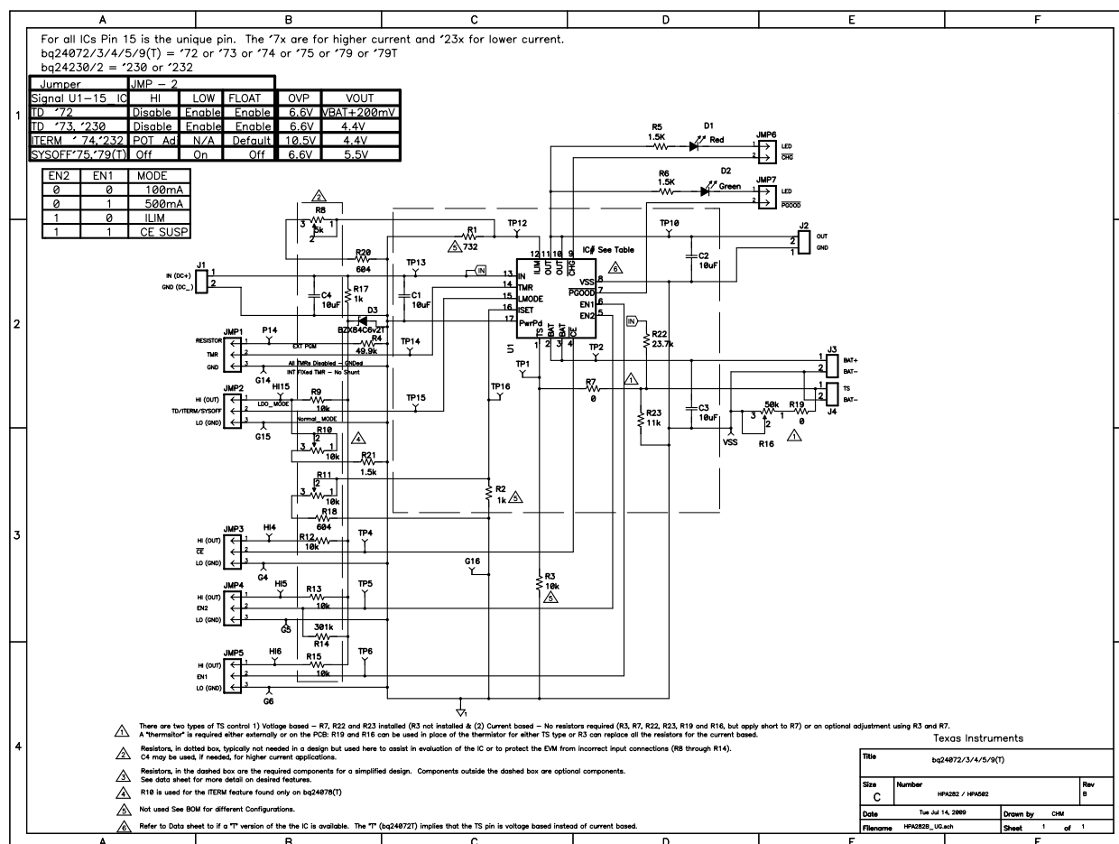
Figure 5. Schematic
