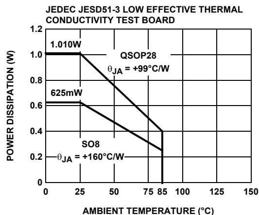
FIGURE 24. PACKAGE POWER DISSIPATION vs AMBIENT TEMPERATURE
