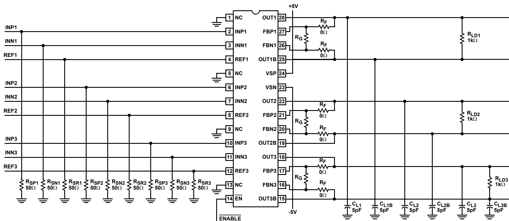
FIGURE 2. EL5374
