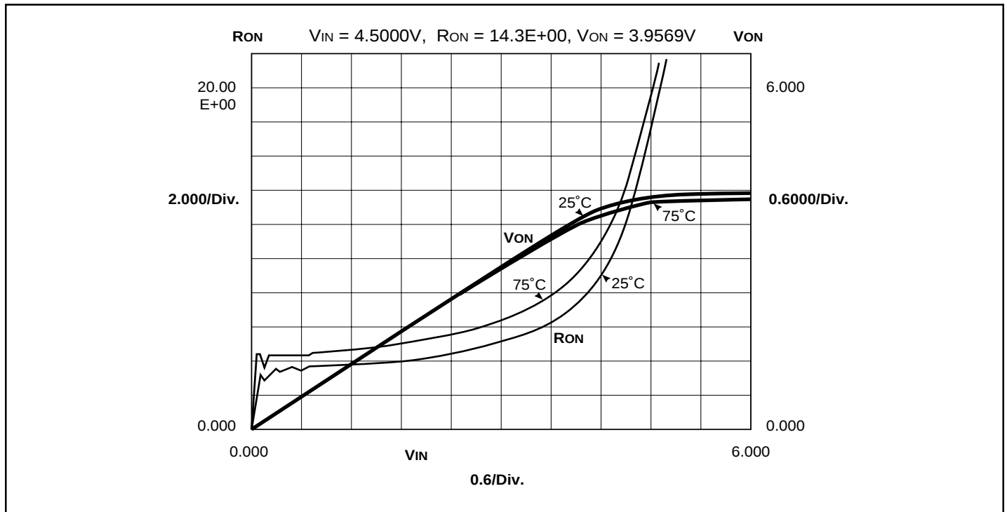
Figure 3. R_{ON} vs Input Voltage over Temperature ( R_{ON} at V_{CC} = 6.1V @ 75^{\circ}C )
