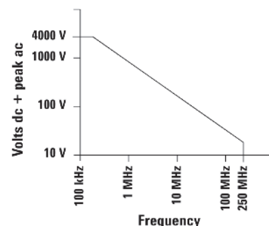
10076B derating curve
