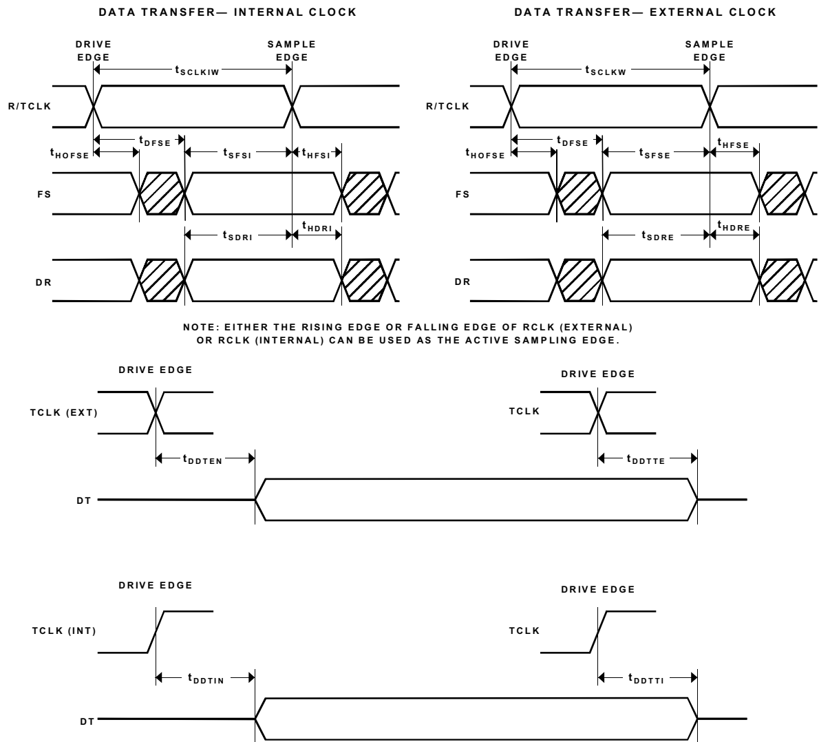
Figure 20. Serial Port (SPORT) Clocks and Data
