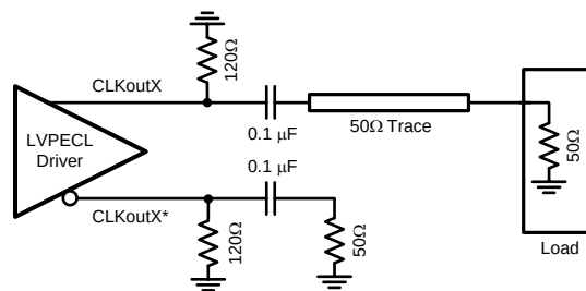
Figure 34. Single-Ended LVPECL Operation, AC Coupling
