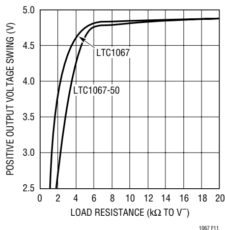
Figure 11. LTC1067/LTC1067-50 Positive Output Voltage Swing vs Load Resistance, 5V Supply
