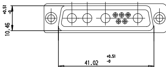
LAYOUT DIMENSIONS (after plating) CONNECTOR SIDE VIEW
