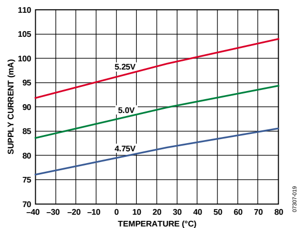
Figure 20. Supply Current vs. Temperature and Supply Voltage (Using 2.6 GHz Matching Components)
