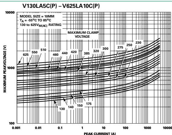
Figure 3. Maximum Clamping Voltage for 10mm Parts
