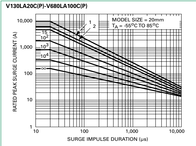
Figure 8. Repetitive Surge Capability for 20mm Parts
