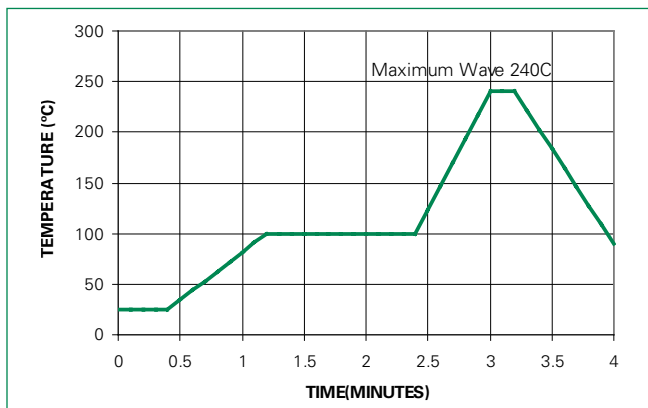
Figure 10. Non Lead-free Profile
