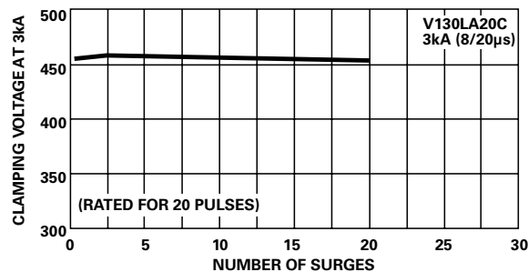
Figure 13 & 14. Typical Repetitive Surge Current Capability of C-III Series MOVs
