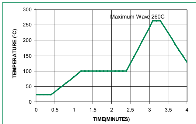
Figure 11. Lead-free Profile
