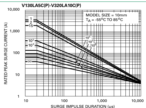
Figure 4. Repetitive Surge Capability for 10mm Parts
