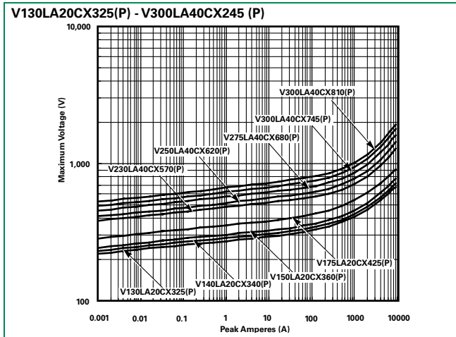
Figure 9. Maximum Clamping Voltage for Low Clamping Voltage Parts
