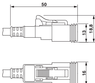
DEUTSCH DT06-2S, top view and side view
