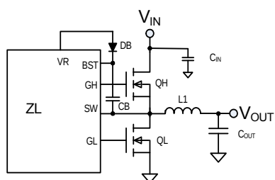
Figure 6. Synchronous Buck Converter
