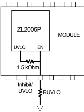
Figure 12. UVLO Circuit
