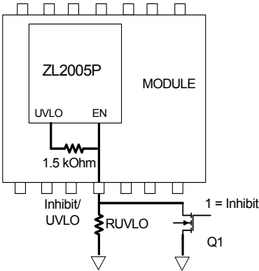
Figure 13. INHIBIT Circuit
