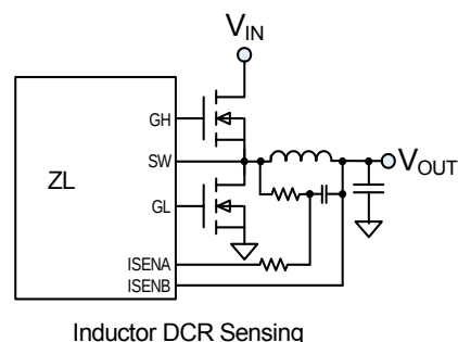
Figure 18. Current Sensing Methods
