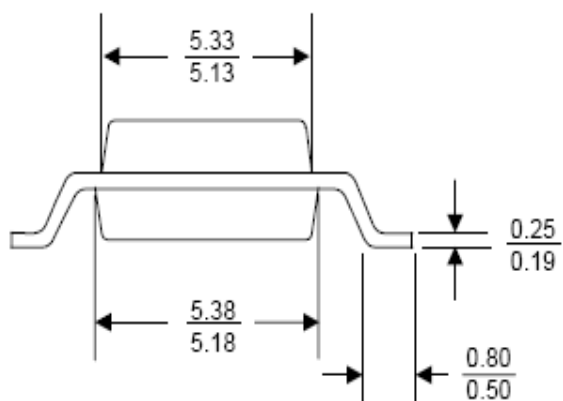
End View
