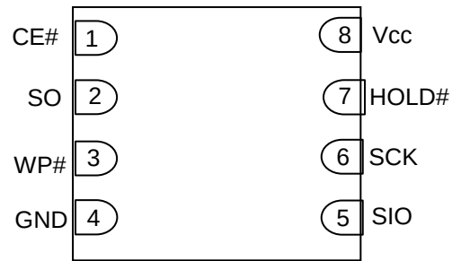
8-Contact WSON
