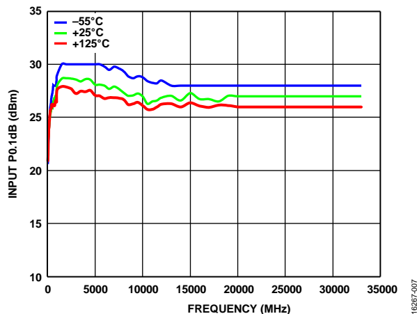
Figure 7. Input P0.1dB vs. Frequency at Minimum Attenuation State and at Various Temperatures
