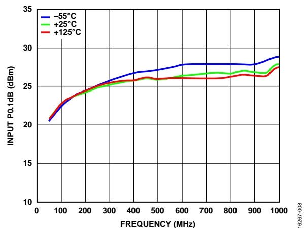
Figure 8. Input P0.1dB vs. Frequency at Minimum Attenuation State and at Various Temperatures (Low Frequency Detail)
