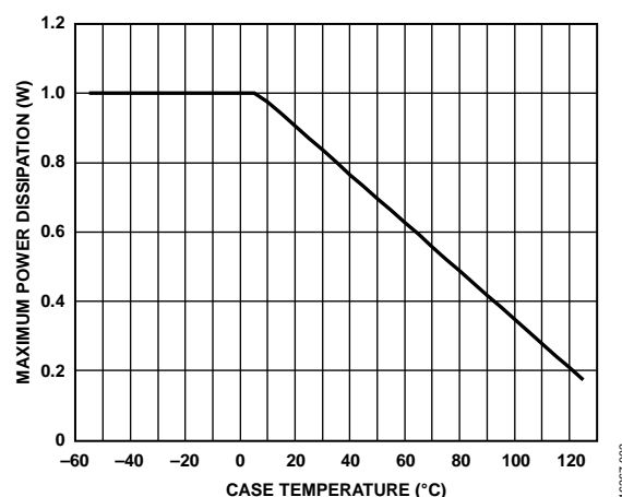
Figure 2. Maximum Power Dissipation vs. Case Temperature ( T_{CASE} )
