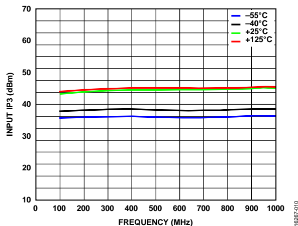
Figure 10. Input IP3 vs. Frequency at Minimum Attenuation State and at Various Temperatures (Low Frequency Detail)
