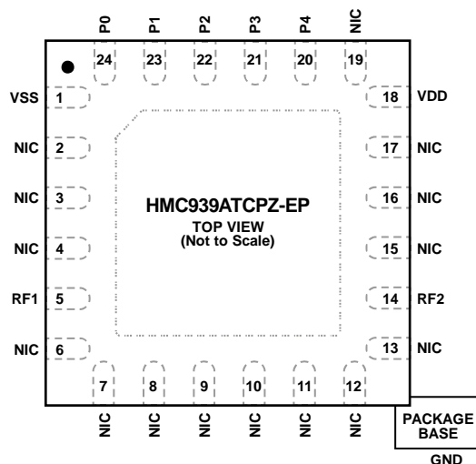
Figure 3. Pin Configuration
