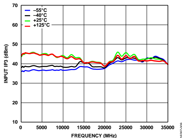
Figure 9. Input IP3 vs. Frequency at Minimum Attenuation State and at Various Temperatures
