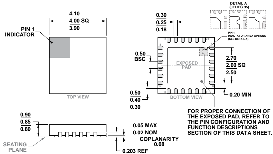
Figure 11. 24-Lead Lead Frame Chip Scale Package [LFCSP] 4 mm × 4 mm Body and 0.85 mm Package Height (CP-24-22)
