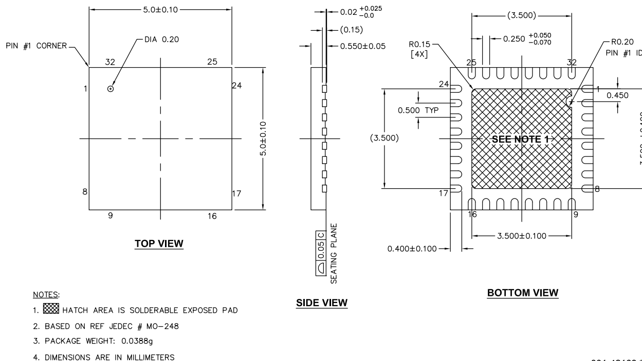
Figure 16. 32-Pin (5x5 mm) QFN
