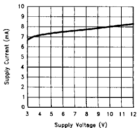
LM7131 Supply Current vs Supply Voltage
