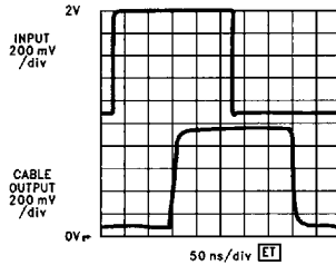
LM7131 Driving 75' RG-59 A_V = +2 @ +3V
