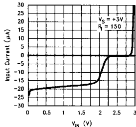
LM7131 Input Current vs Input Voltage @ 3V
