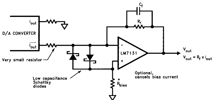
FIGURE 16. D/A Output Amplifier
