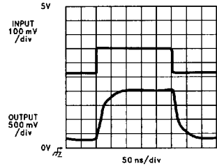
LM7131 Cable Driver A_V = +10 @ +3V
