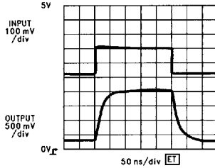
LM7131 Cable Driver A_V = +10 @ +5V
