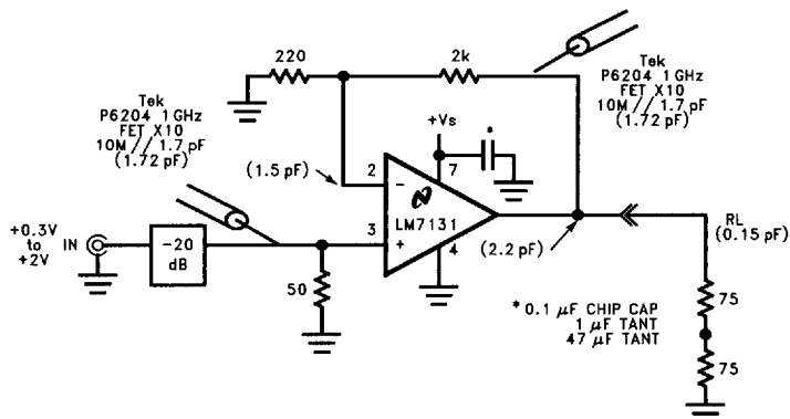
FIGURE 5. Cable Driver Gain of 10 A_v = +10
