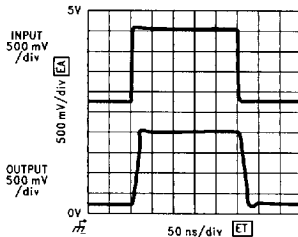
LM7131 Cable Driver A_V = +1 @ +3V
