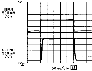
LM7131 Cable Driver A_V = +2 @ +5V
