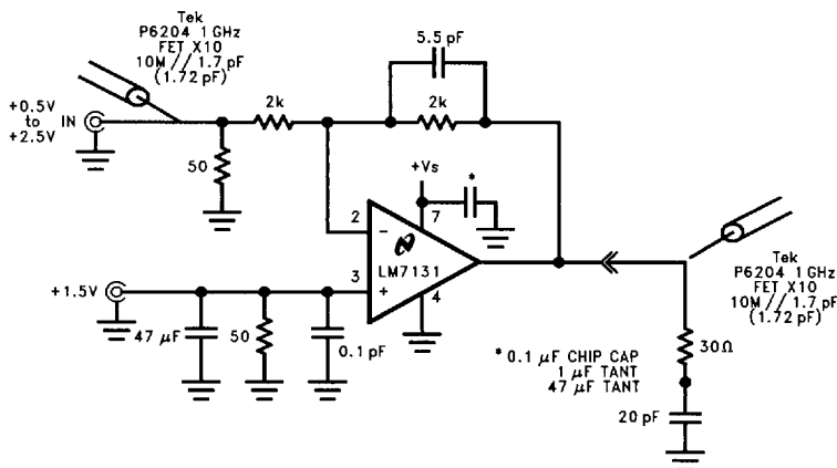
FIGURE 6. Flash A/D A_V = -1
