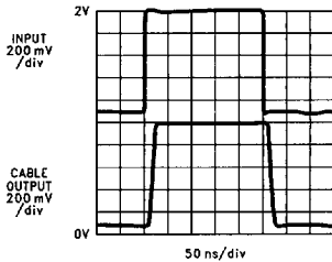
LM7131 Driving 5' RG-59 A_V = +2 @ +3V
