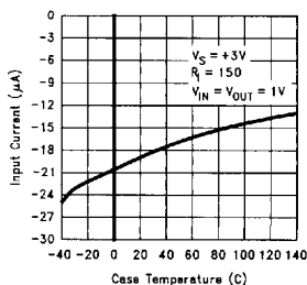
LM7131 Input Current vs Temperature @ 3V
