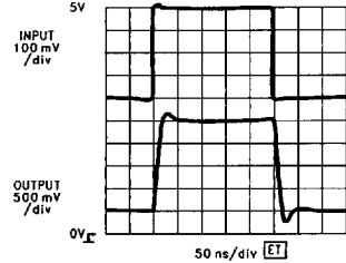
LM7131 Driving Flash A/D Load A_V = +5 @ +5V
