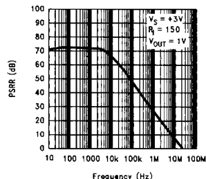
LM7131 PSRR vs Frequency @ 3V
