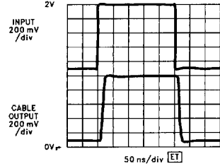
LM7131 Driving 5' RG-59 A_V = +2 @ +5V
