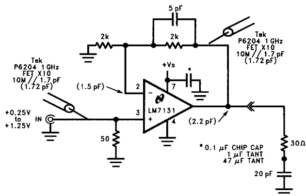
FIGURE 8. Flash A/D A_y = +2
