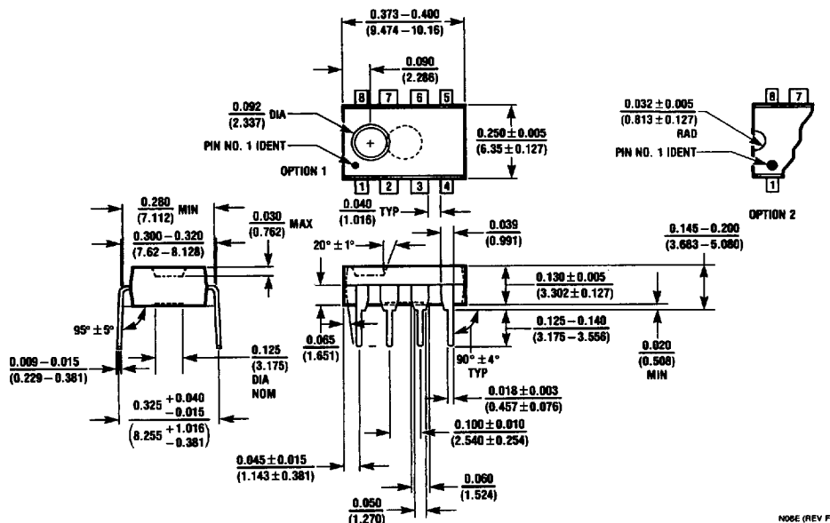
8-Pin Molded DIP 8-Lead (0.300" Wide) Molded Dual-In-Line Package Order Package Number LM7131ACN or LM7131BCN NS Package Number N08E
