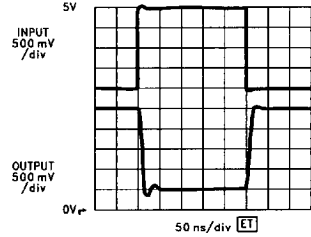
LM7131 Driving Flash A/D Load A_V = -1 @ +5V
