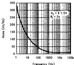
LM7131 Voltage Noise vs Frequency @ 3V
