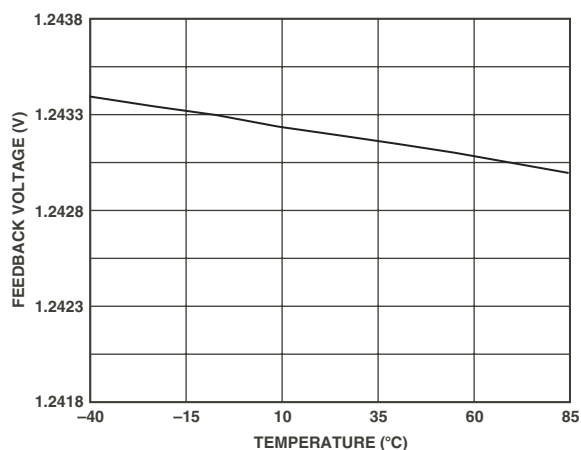
TPC 6. Feedback Voltage vs. Temperature
