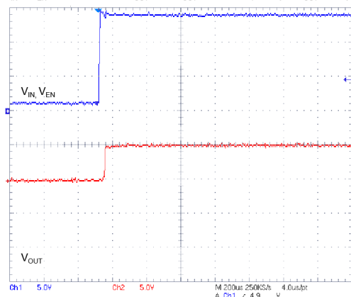
Figure 39. Start-up transient ( I_{OUT} = 400\text{ mA} )
