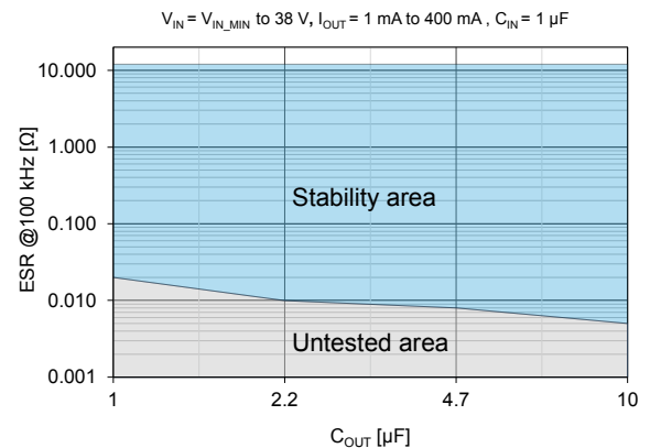
Figure 27. Stability plan
