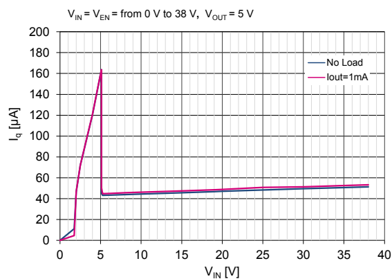
Figure 26. Quiescent current vs. input voltage
