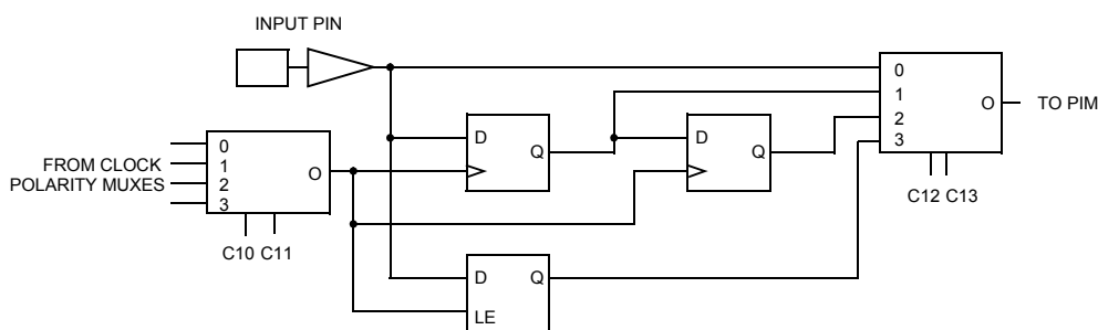
Figure 3. Input Macrocell
