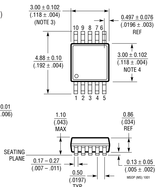
MS Package 10-Lead Plastic MSOP (Reference LTC DWG # 05-08-1661)
