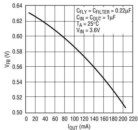
Feedback Voltage vs I_{OUT}
