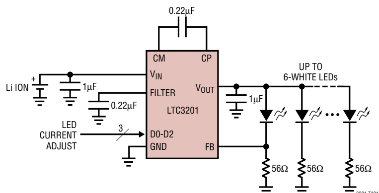
Ultralow Noise White LED Driver with Adjustable Current Control
