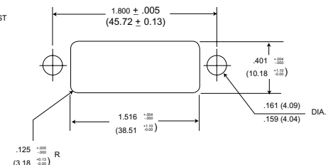
Dimensions for Rear Panel Mounting
